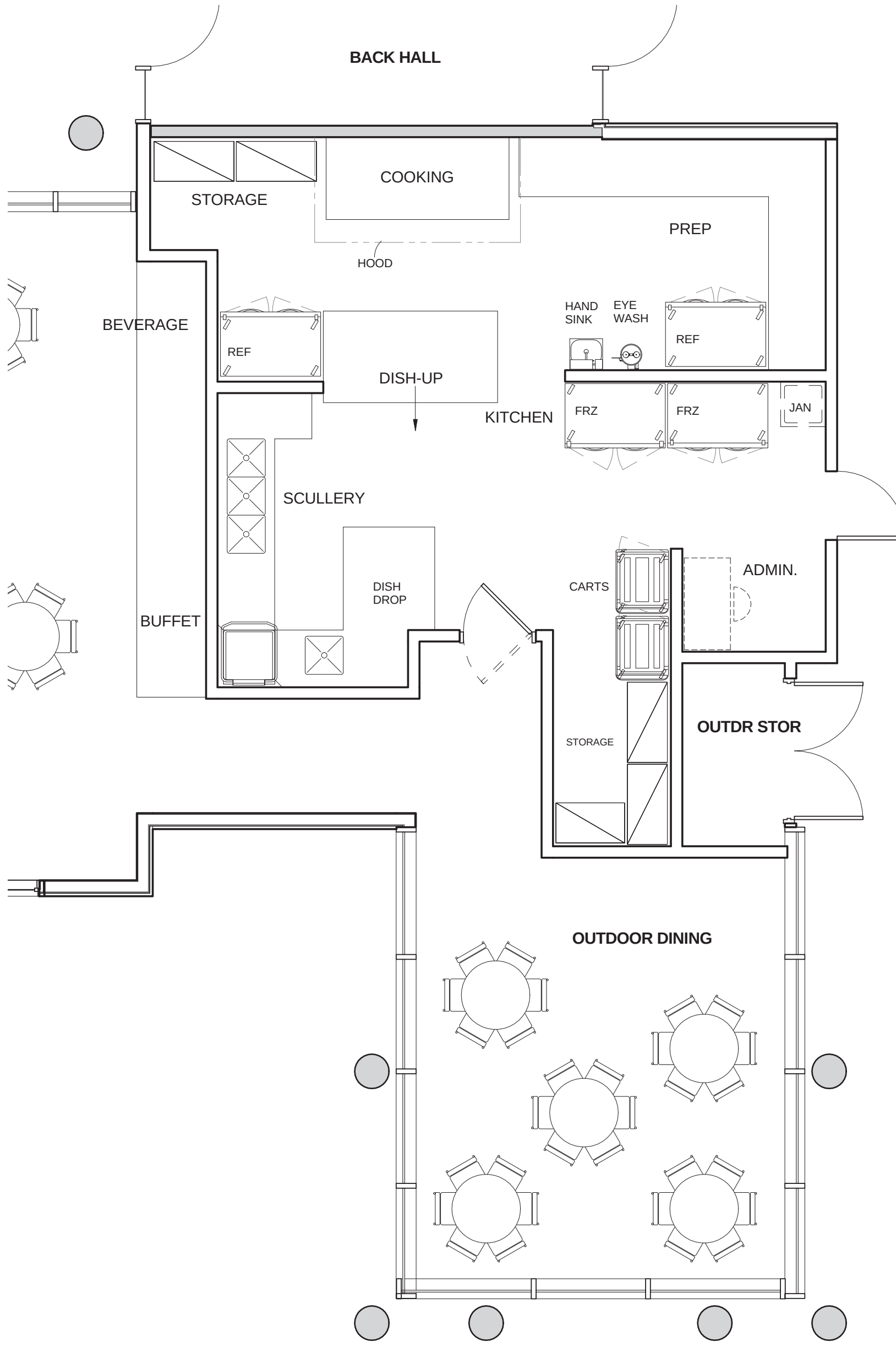
Enlarged Kitchen Plan // nts
