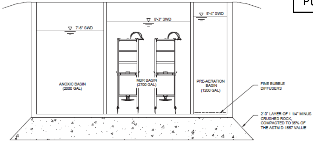
MBR TANK SECTION
