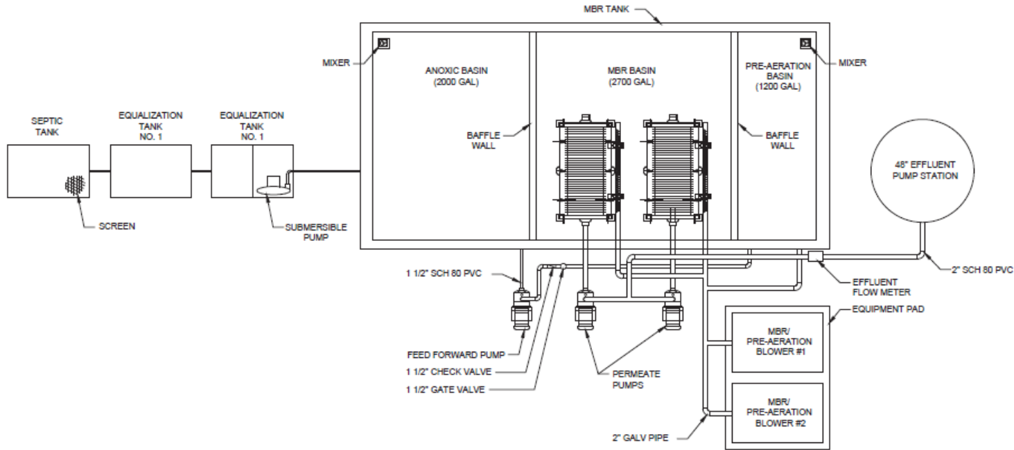
MBR SYSTEM PLAN
